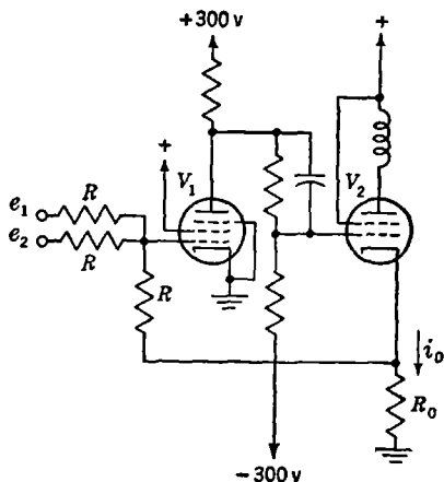
FIG. 10-12.—Direct-coupled feedback circuit for producing an output current i_o proportional to e_1 + e_2 . R \gg R_0 .
